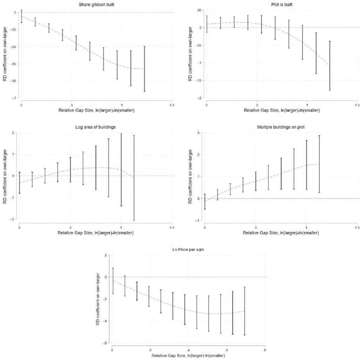
Figure A.6: RD coefficients by gap size
